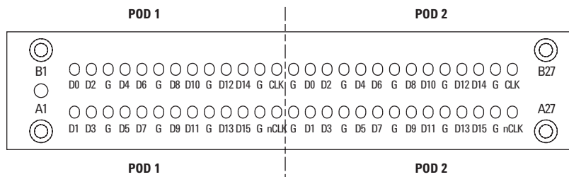
Figure 8.16. Pinout
