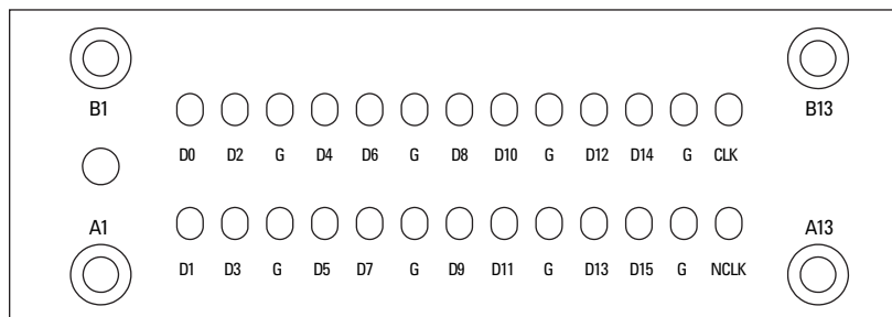
Figure 8.15. Pinout
