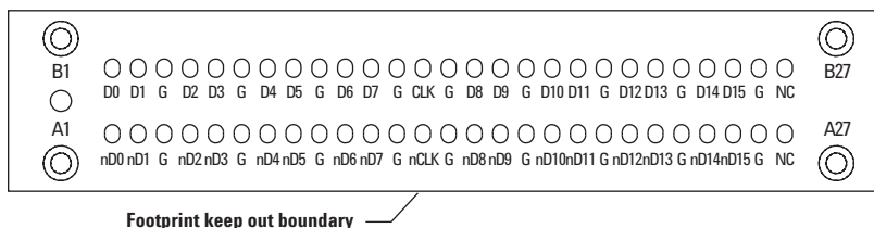
Figure 8.14. Pinout
