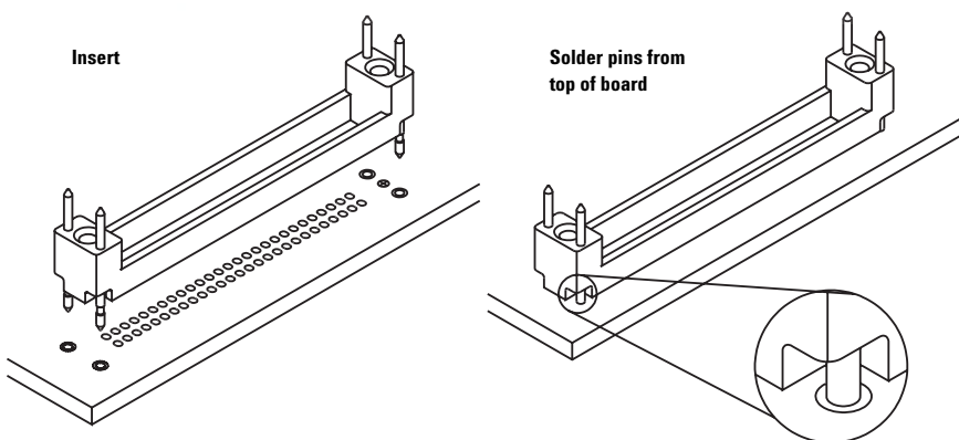
Figure 5.1. "Top-side" mountable retention module.
