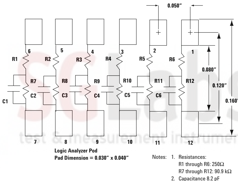
Figure 5.26. Recommended PC board pattern for 5062-7396 surface mount isolation network
