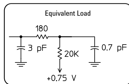
Figure 10.7. E5380A input equivalent load, including 38-pin connector
