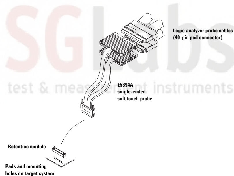
Figure 5.2. Agilent E5394A soft touch probe connection
