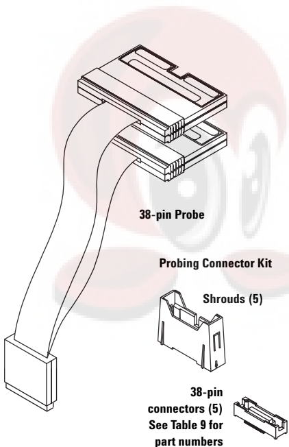
Figure 10.1. Agilent E5380A probe
