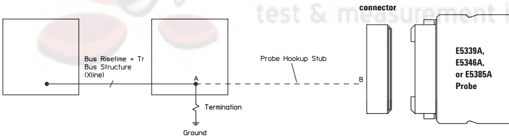
Figure 5.22. Agilent E5339A, E5346A, and E5385A design rules
