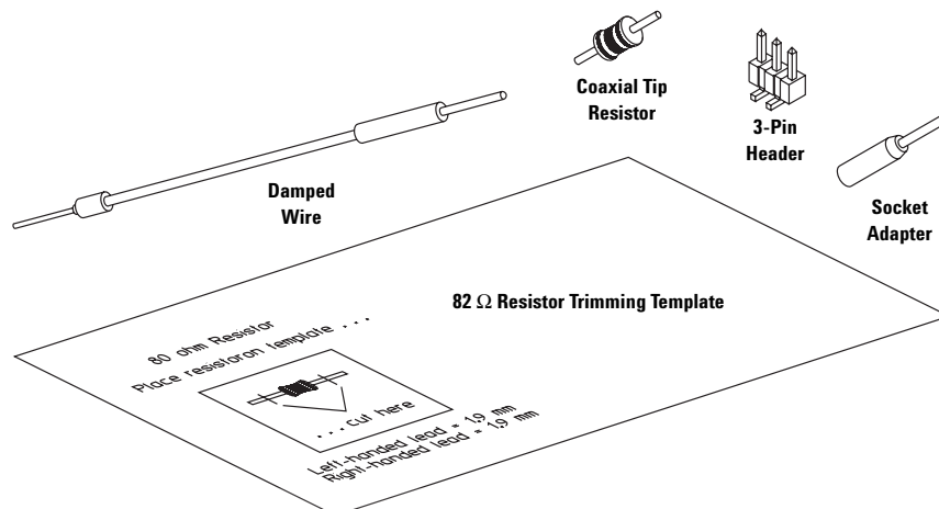
Figure 11.4. E5381A differential flying-lead probe set accessories
