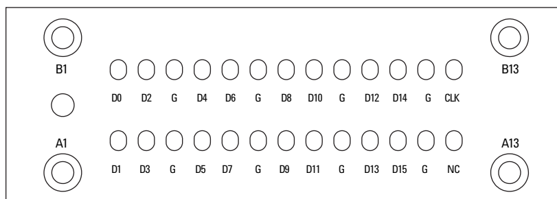
Figure 5.13. Pinout
