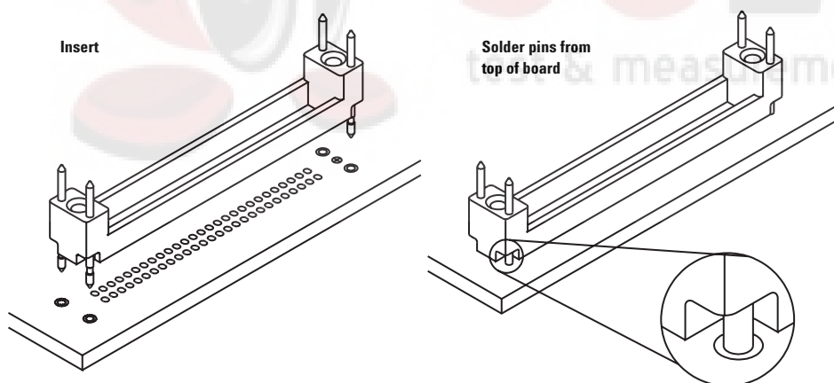
Figure 8.1. "Top-side" mountable retention module.
