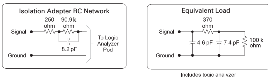
Figure 7.3. Isolation adapter (01650-63203) and equivalent load
